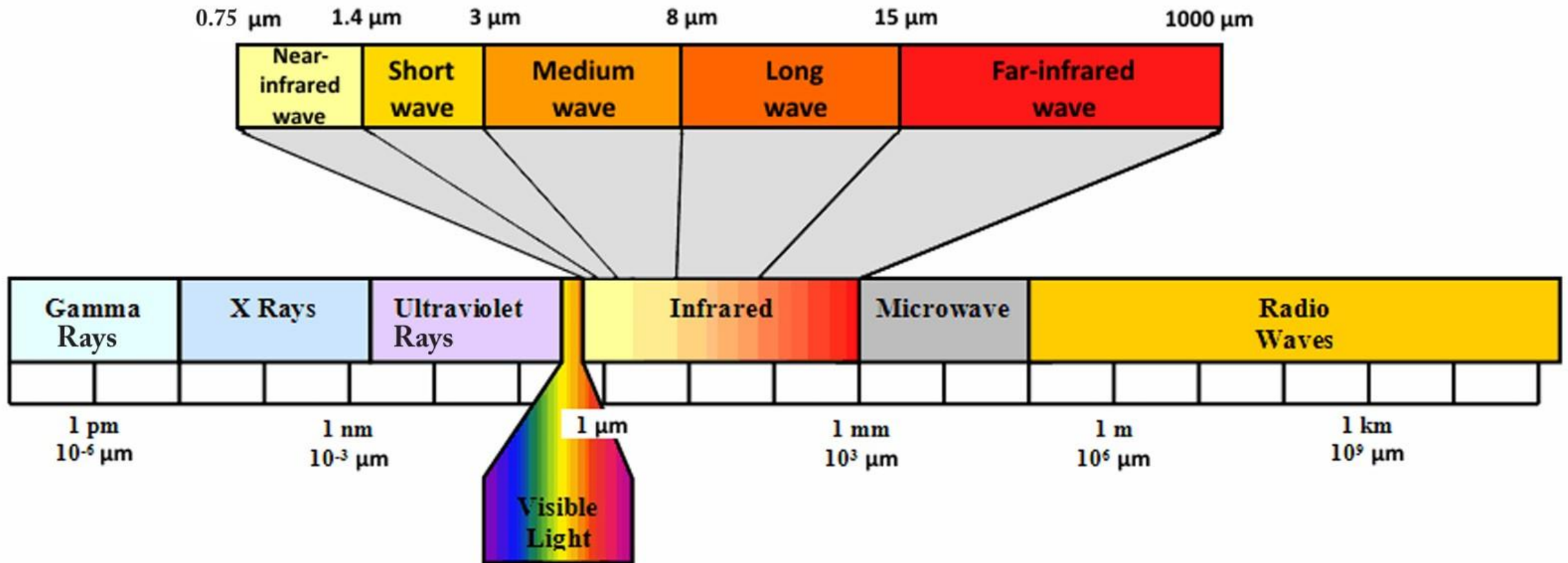
Figure 1. Electromagnetic spectrum. Thermal Infrared is part of Longwave Infrared region between 8-14 μm.
